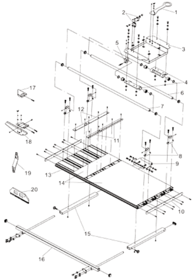
ALPHA® ECOCUTTER TABLE SCHEMATIC (ECC-TABLE)
